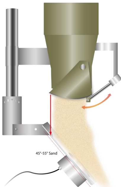
Sand: Angle baffle plate 45° to 55°
