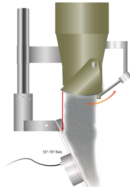
Gravel: Angle baffle plate 55° to 70°
